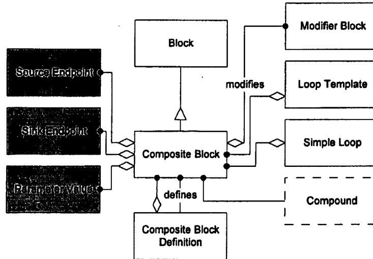
Figure 90 - Composite Block object model
